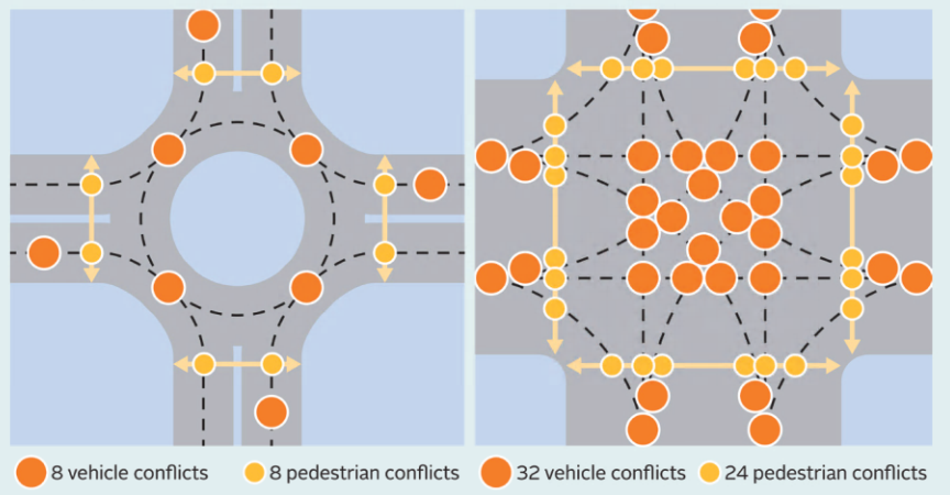
These images compare the pedestrian and vehicle conflict points at a traditional intersection versus a roundabout.
