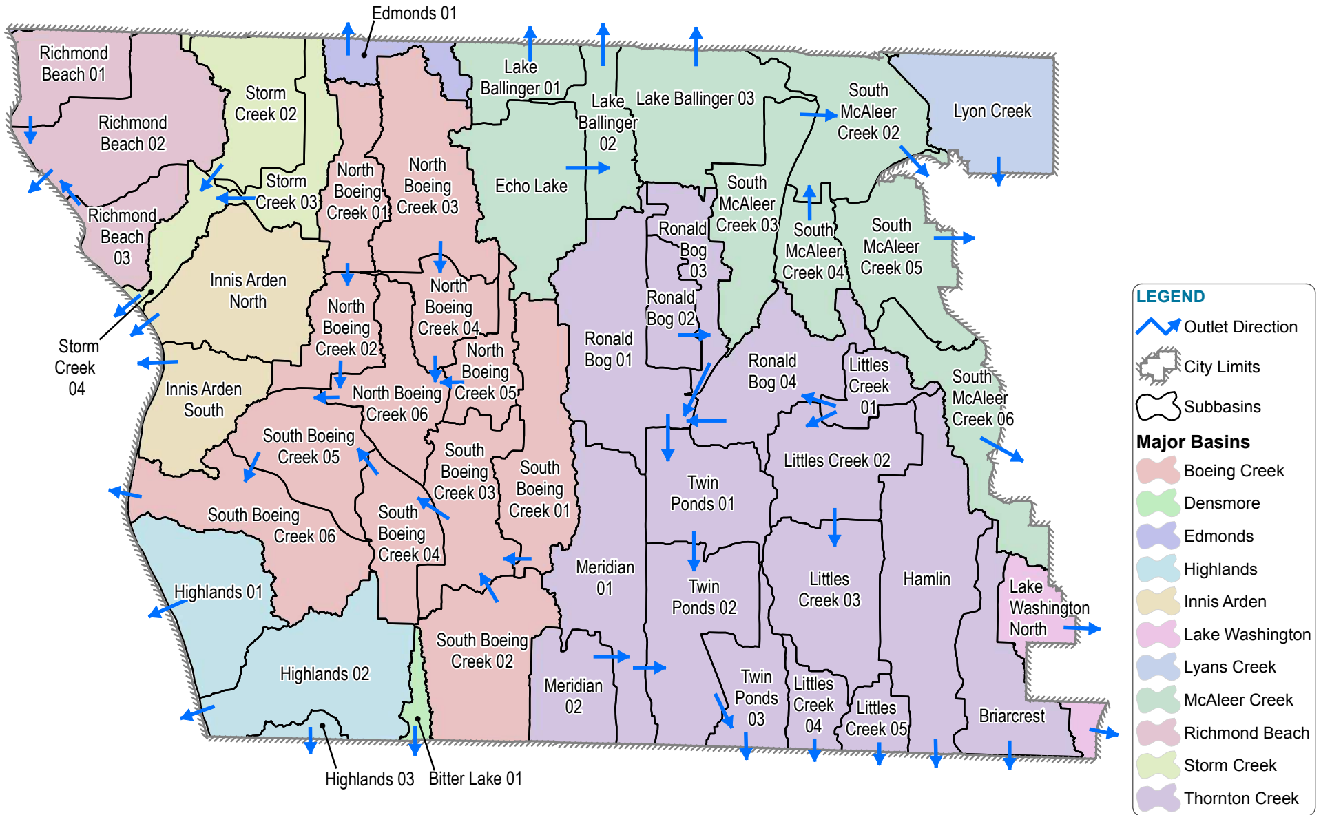
Figure 4-1 Newly Delineated Subbasins and Connectivity
