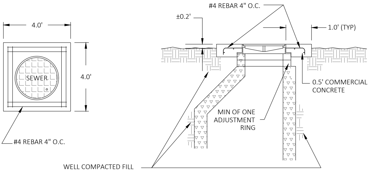
MANHOLE OUTSIDE PAVED AREA
