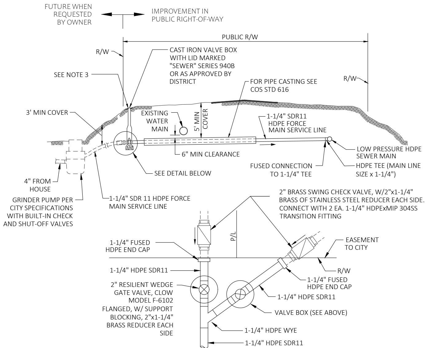
DOUBLE SERVICE DETAIL
