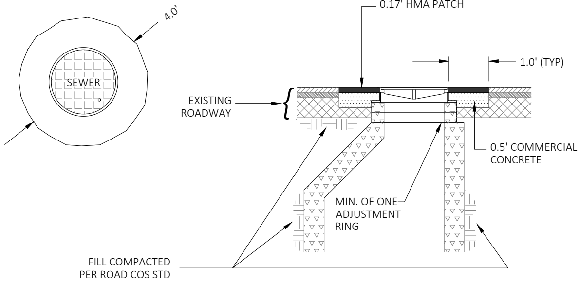
MANHOLE IN PAVED AREA
