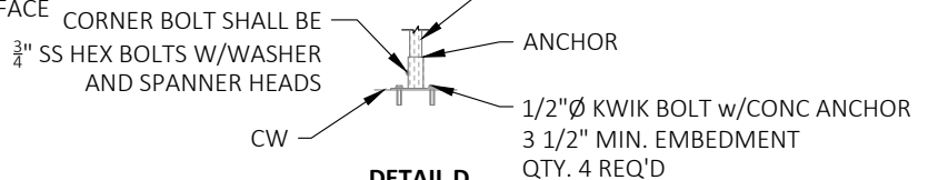
DETAIL D SURFACE MOUNT INSTALLATION
