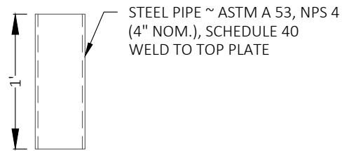
POST SLEEVE
