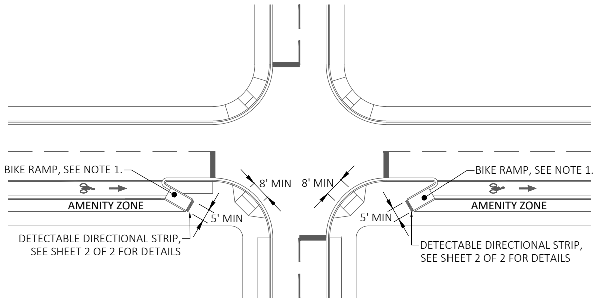
BIKE RAMP TO/FROM SIDEWALK GRADE WITH AMENITY ZONE
