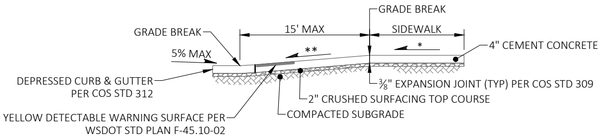
SECTION VIEW
