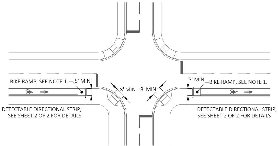
BIKE RAMP TO/FROM SIDEWALK GRADE WITHOUT AMENITY ZONE
