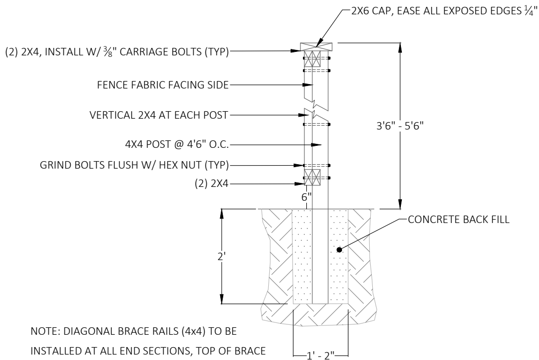
SECTION
