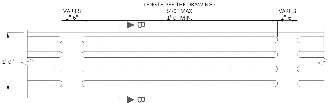
DETECTABLE DIRECTIONAL STRIP - SURFACE APPLIED MMA *MMA STRIP ONLY ALLOWED WHEN RETROFITTING EXISTING RAMP
