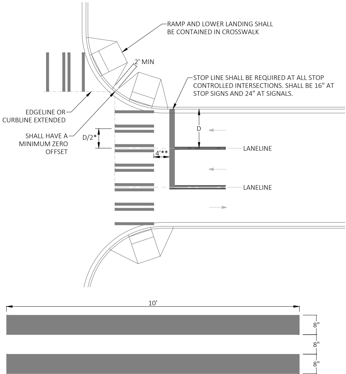
CROSSWALK DETAIL
