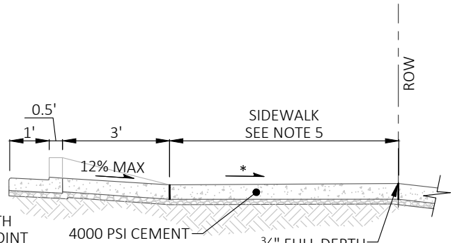
SECTION A-A (REVERSE SLOPE)
