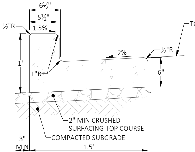
TYPE A CURB AND GUTTER
