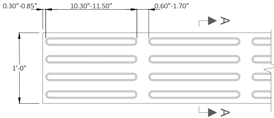
DETECTABLE DIRECTIONAL STRIP - CAST-IN-PLACE *CAST IN PLACE STRIP IS PREFERRED
