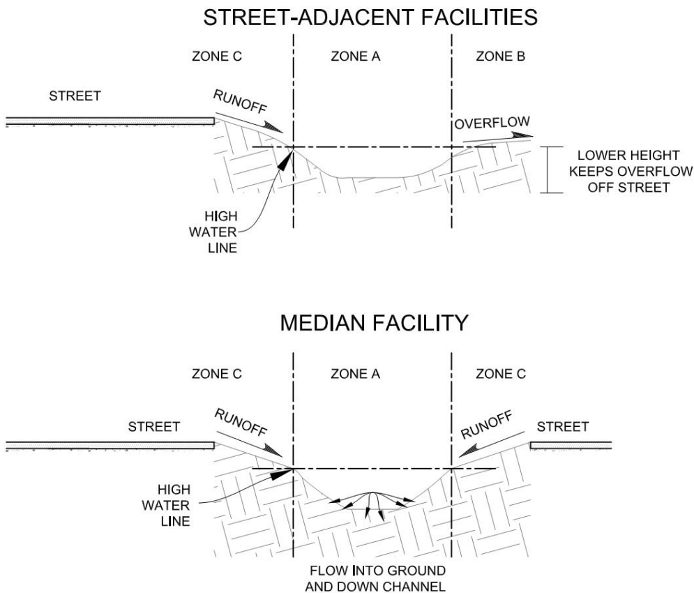
Figure K1. Bioretention Planting Zones
