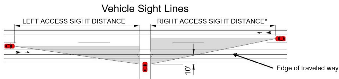
Figure 4. Driveway Sight Triangles
