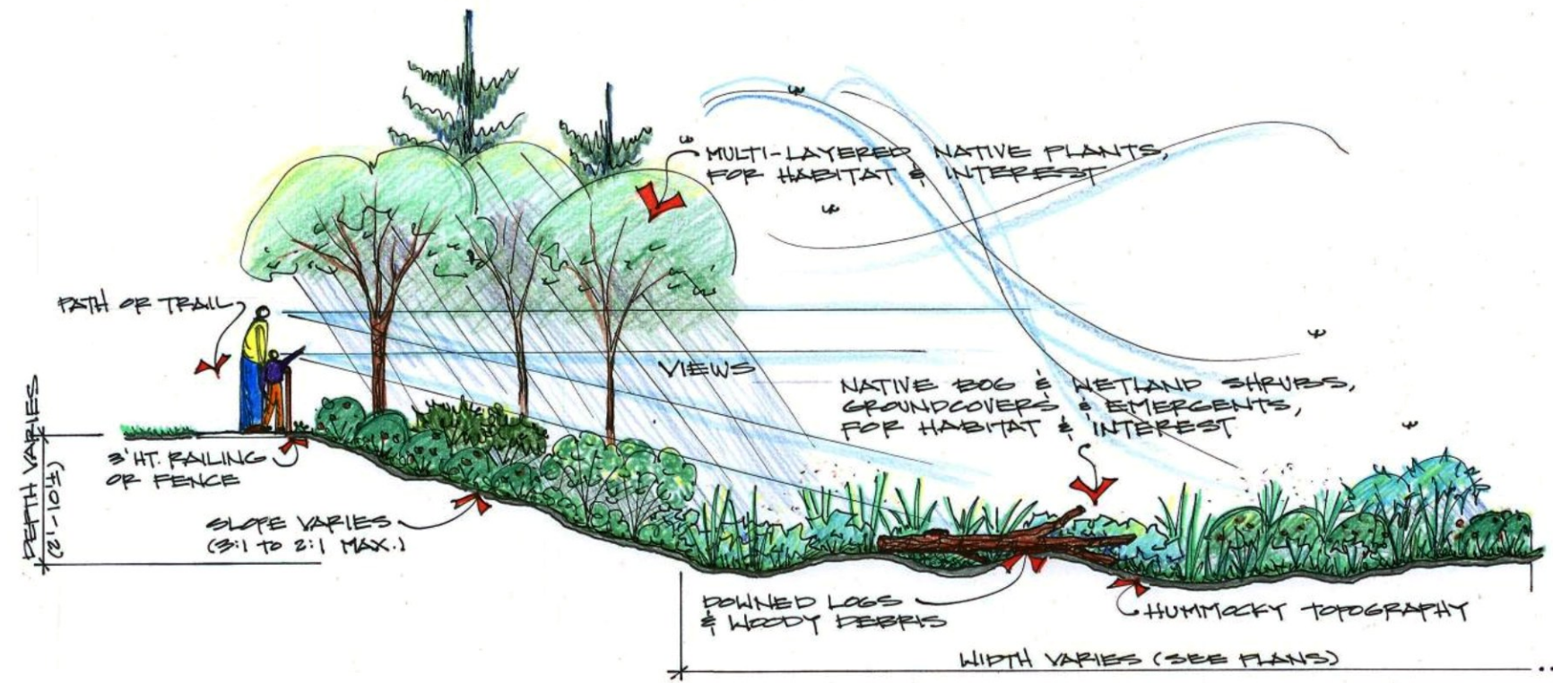
TYPICAL NATURAL DRAINAGE SYSTEM: SECTION & LANDSCAPE 1/4" = 1'-0"±
