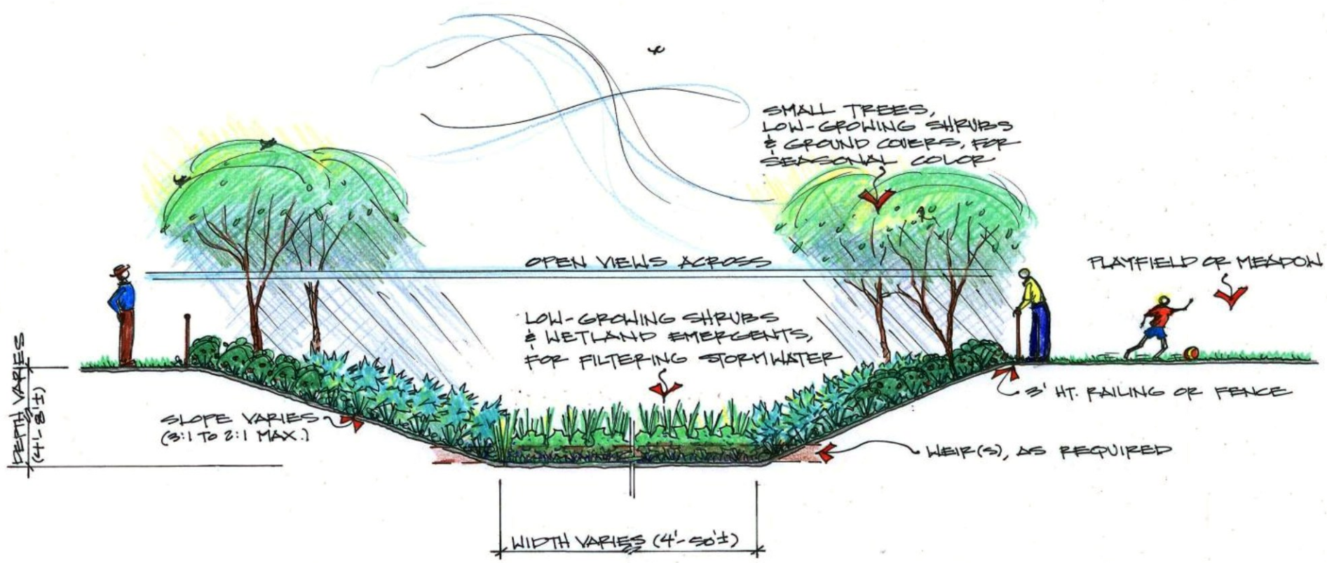
TYPICAL NATURAL DRAINAGE SYSTEM: SECTION & LANDSCAPE 1/4" = 1'-0"±
