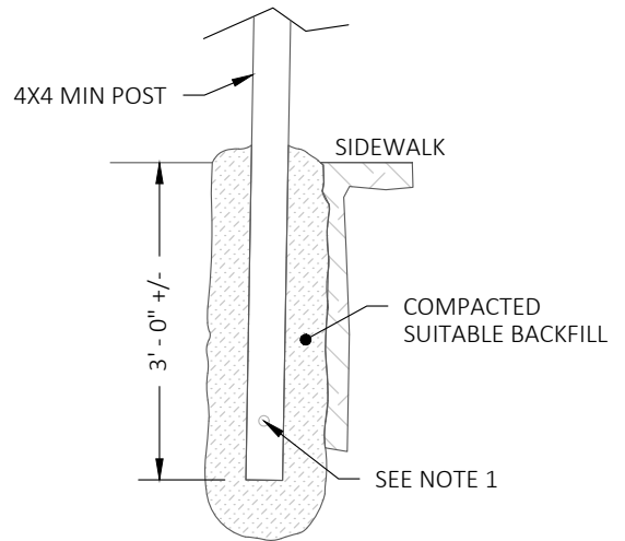
DETAIL C
