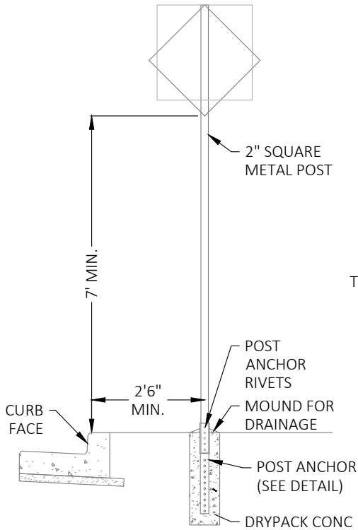
DIRECT BURIAL INSTALLATION
