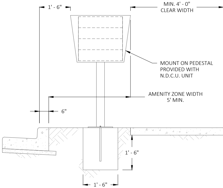
SIDE VIEW
