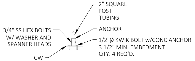
DETAIL D SURFACE MOUNT INSTALLATION
