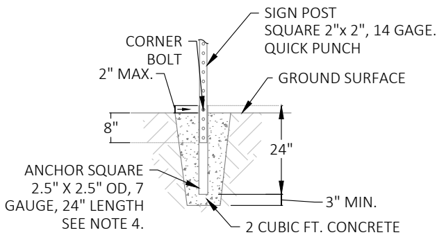
DETAIL C SQUARE METAL POST
