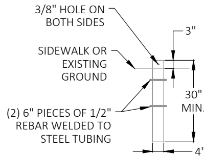
DETAIL B ANCHOR DETAIL
