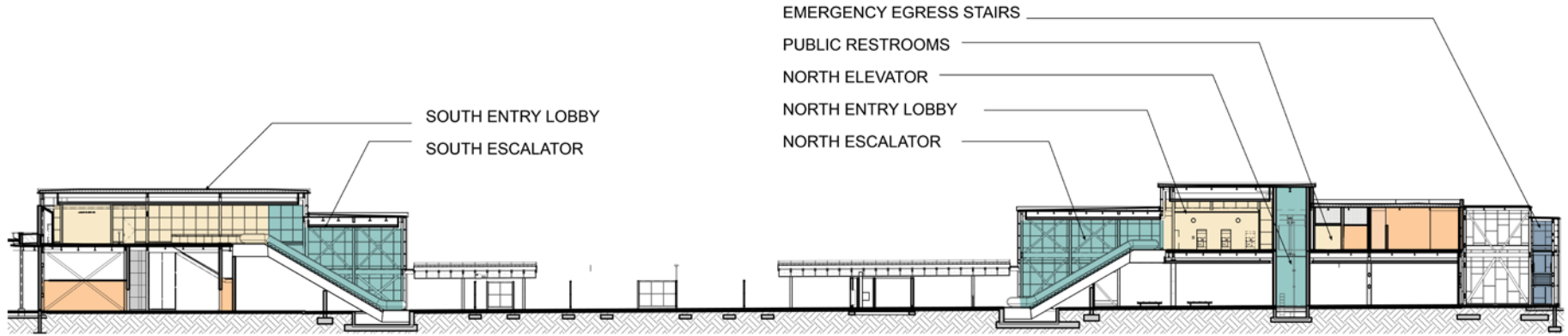
NE 185TH ST STATION: LONGITUDINAL SECTION
