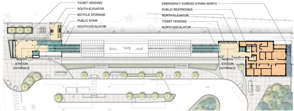
NE 185TH ST STATION: PLAZA LEVEL PLAN
