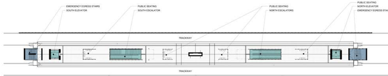
145th ST. STATION: PLATFORM LEVEL PLAN
