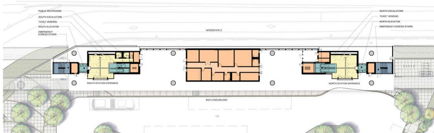
145th ST. STATION: PLAZA LEVEL PLAN
