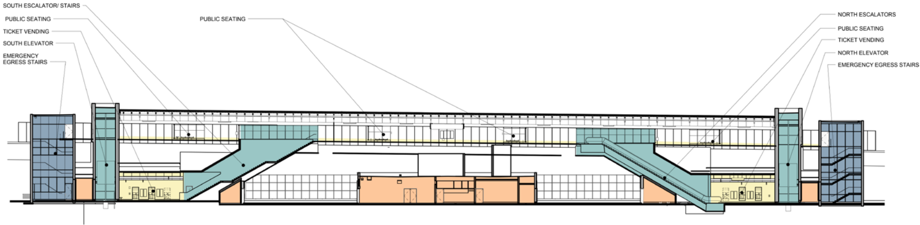
145th ST. STATION: LONGITUDINAL SECTION
