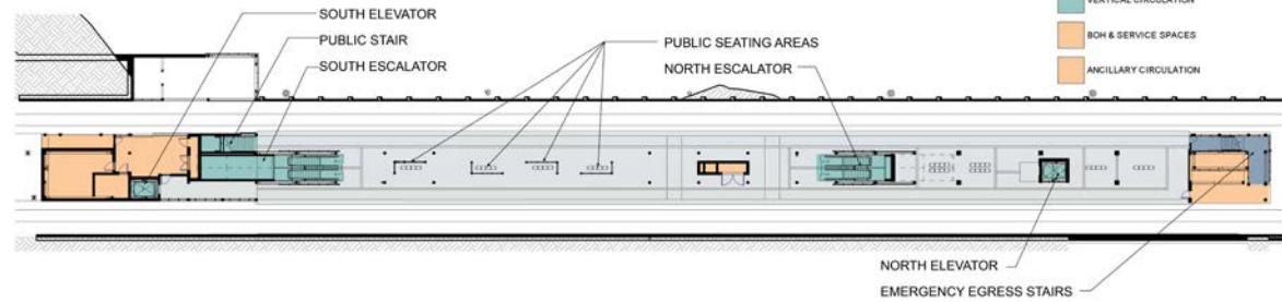
NE 185TH ST STATION: PLATFORM LEVEL PLAN
