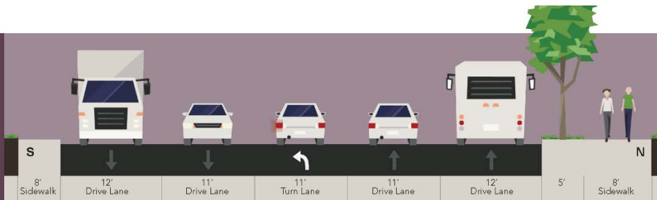
TYPICAL INTERSECTION BETWEEN AURORA AND I-5
