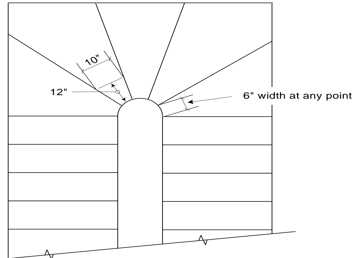
Typical winder detail. Minimum stairway width of 36 inches must be maintained.
