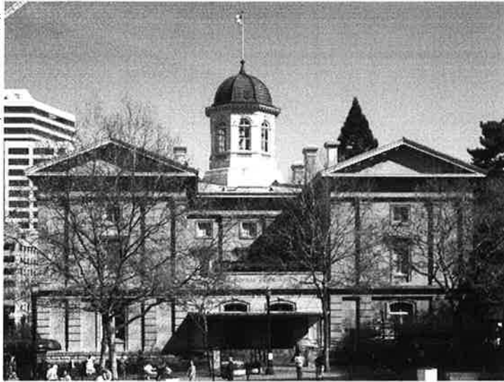
Built in 1875, Pioneer Courthouse in Portland (OR) was rehabilitated in 2005. A seismic base isolation system was installed, which decouples the superstructure from the foundation during an earthquake: The foundation absorbs most of the shaking.
